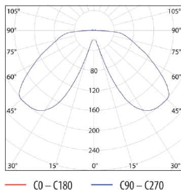
PARK LED 40W XP-G
